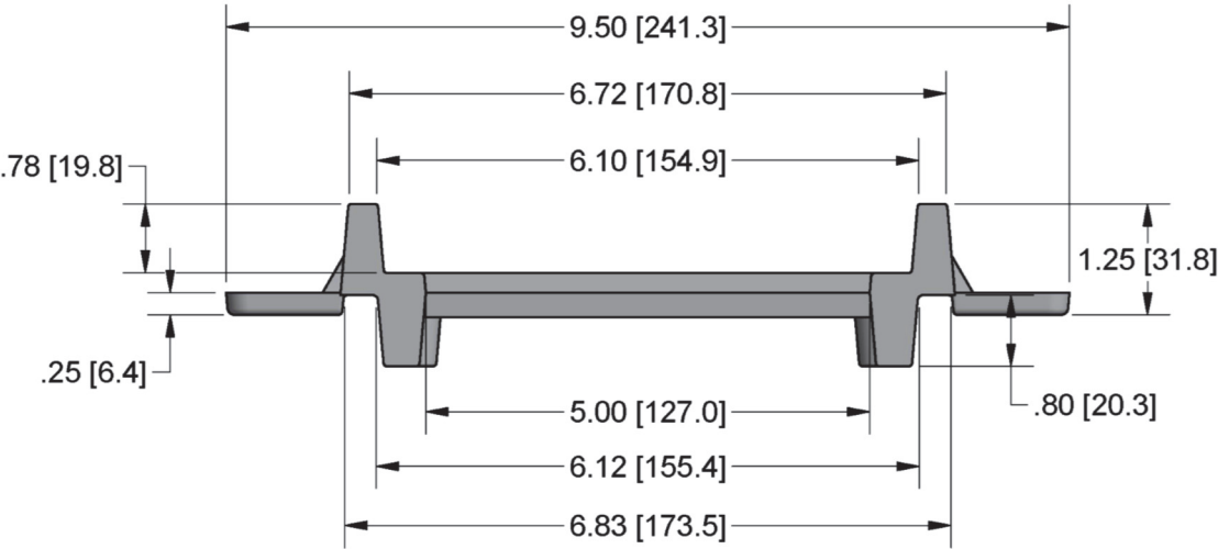
Ductile Iron Top Frame—24 In. Long
